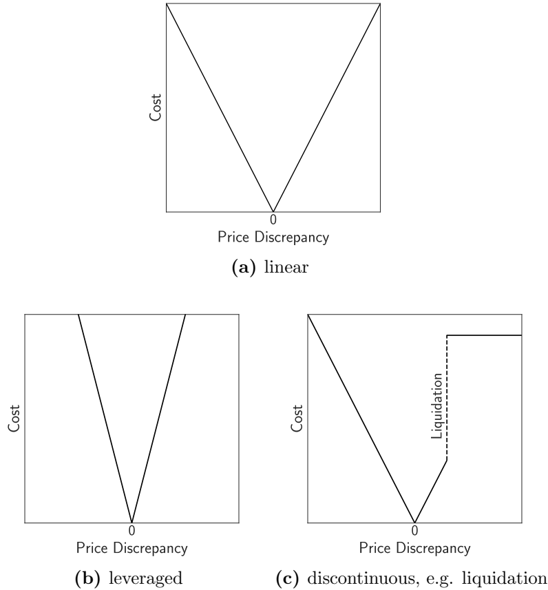
Figure 8: The data from the dAPI can be used in different systems, and the linearity and continuity in the mechanics of these systems decide on how sensitive they are to errors in input data.
